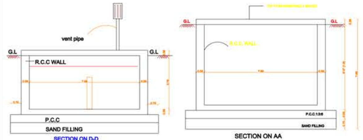
SECTION ON D-D
