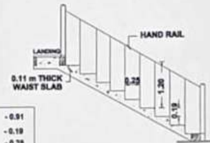
STAIRCASE DETAIL
