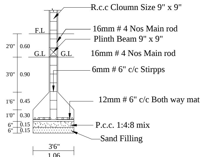
COLUMN DETIAL
