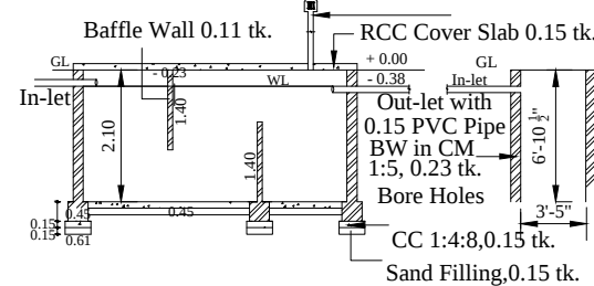
SEPTIC TANK & SOAK PIT
