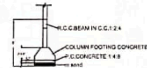
FOUNDATION DETAILS
