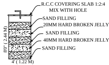
RAIN WATER HARVEST UNIT
