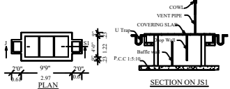
SEPTIC TANK DETAILS
