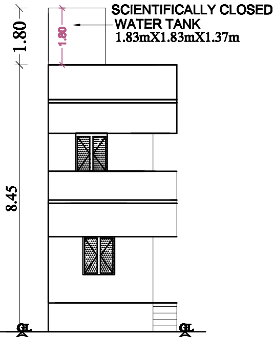
FRONT ELEVATION
