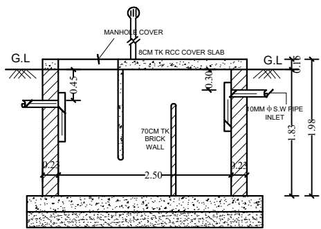
SECTION OF SEPTIC TANK N.T.S
