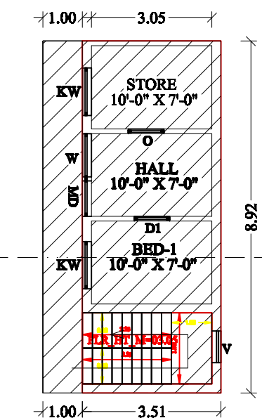
EXSITING FIRST FLOOR PLAN
