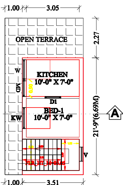
PROPOSED ADDITINAL SECOND FLOOR PLAN
