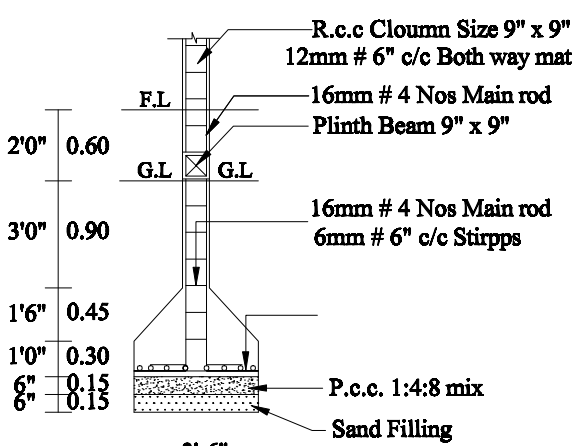
COLUMN DETIAL NOT TO SCALE
