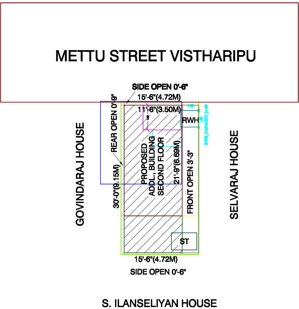
SITE PLAN (SCALE: 1CM : 1M)
