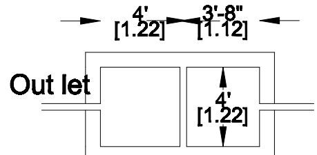
Plan SEPTIC TANK DETAIL
