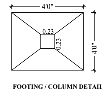
FOOTING / COLUMN DETAIL
