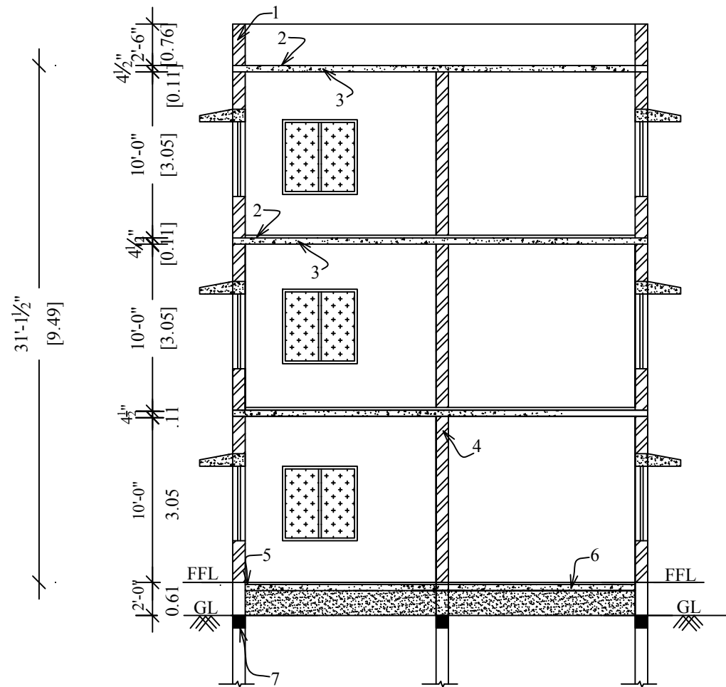
SECTION ON "JS"
