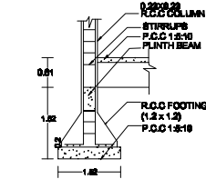
COLUMN DETAILS Size of column = 0.23m x 0.23m Not to scale
