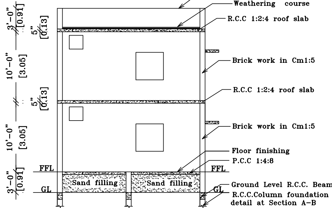
SECTION ON 'SS'
