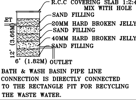
VASTE WATER RECYCLE UNIT
