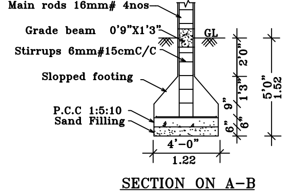
COLUMN DETAILS SCALE : 1"=4'
