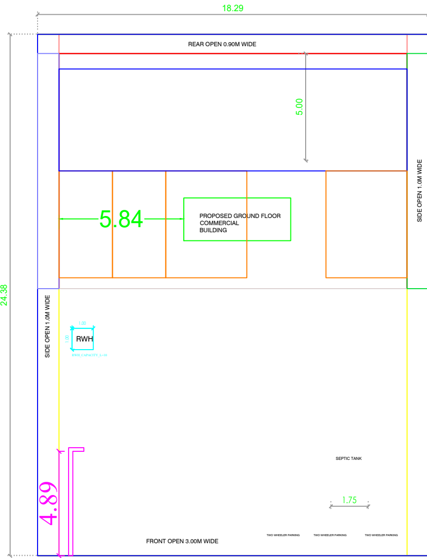
SITE CUM FLOOR DETAILS
