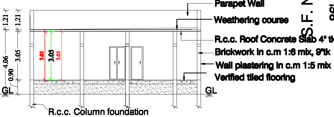
SECTION NN (SCALE: 1CM : 1M)
