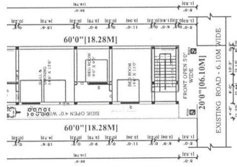
PRO.GROUND FLOOR PLAN
