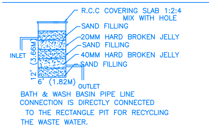
WASTE WATER RECYCLE UNIT
