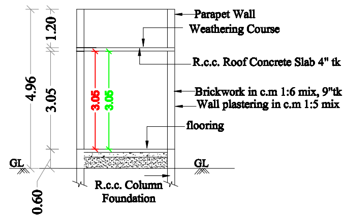
SECTION NN
