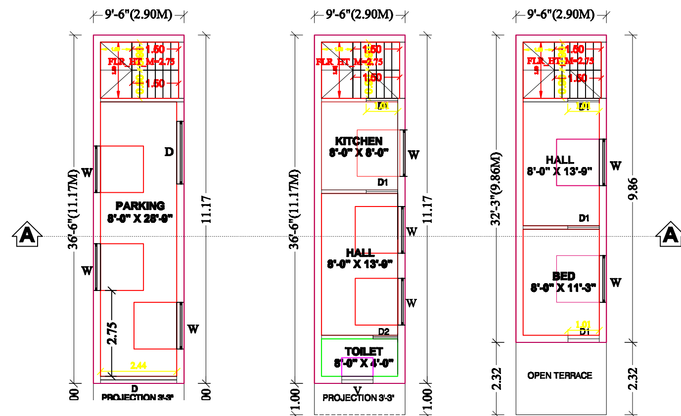
IN FIRST FLOOR PLAN SECOND FLOOR PLAN
