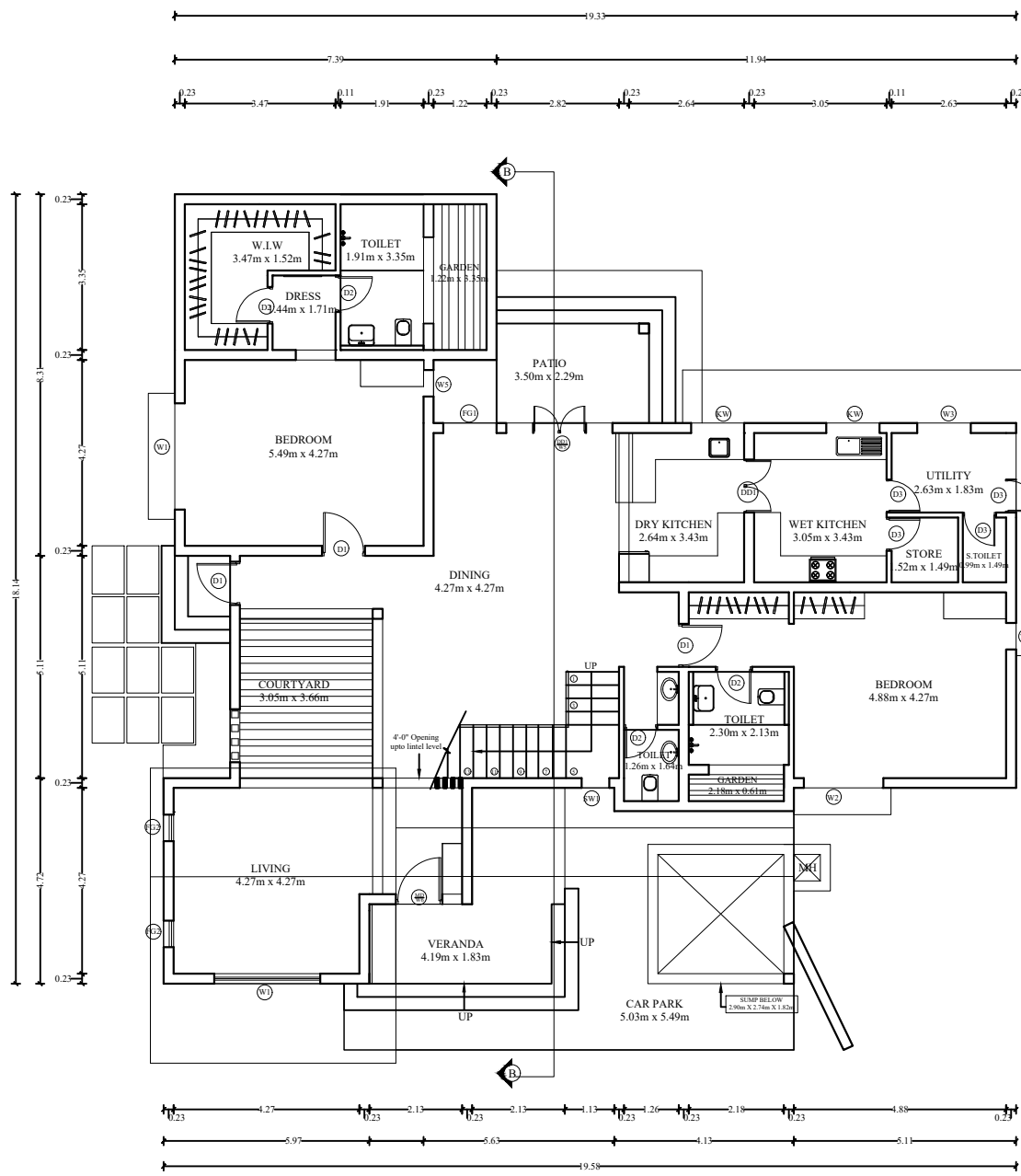
FLOOR PLAN
