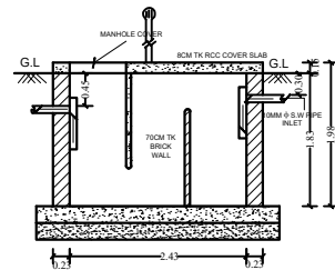
SECTION OF SEPTIC TANK N.T.S
