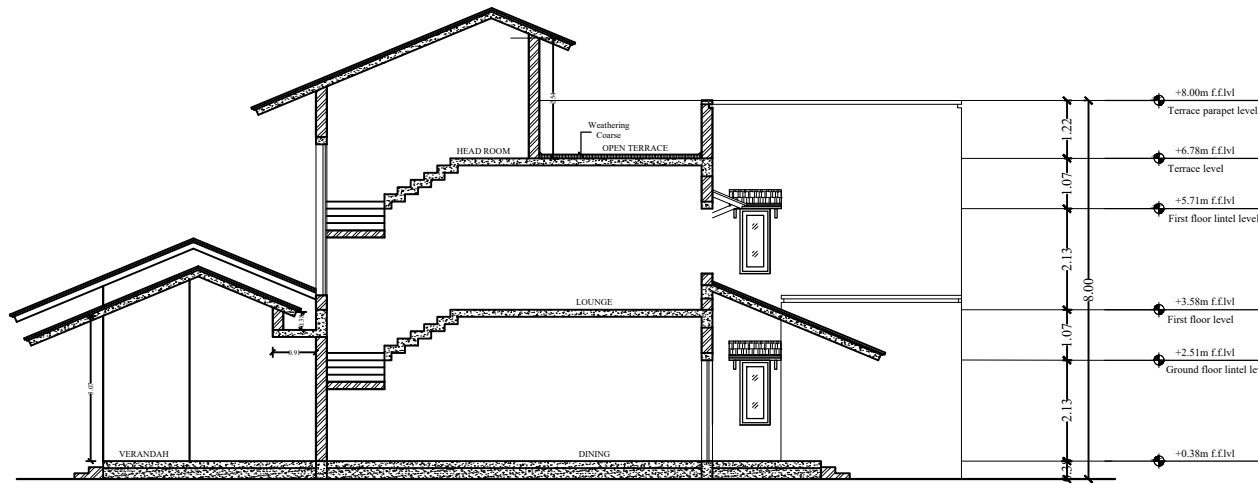
SECTION-BB
