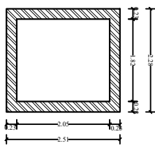
PLAN OF OVER HEAD WATER TANK N.T.S
