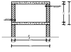
SECTION OF OVER HEAD WATER TANK N.T.S
