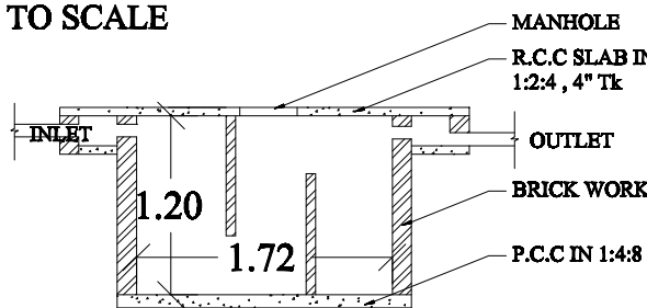
SECTION - CD
