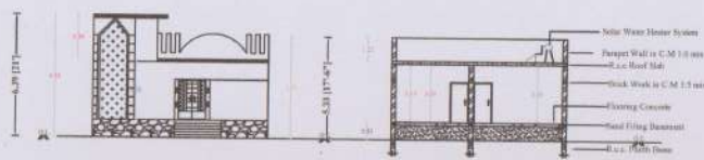
FRONT ELEVATION
