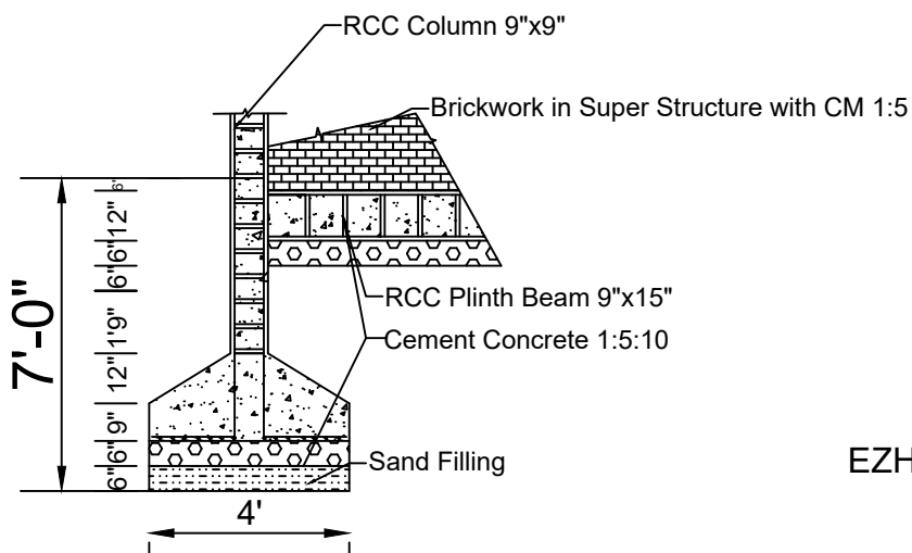
FOUNDATION DETAILS
