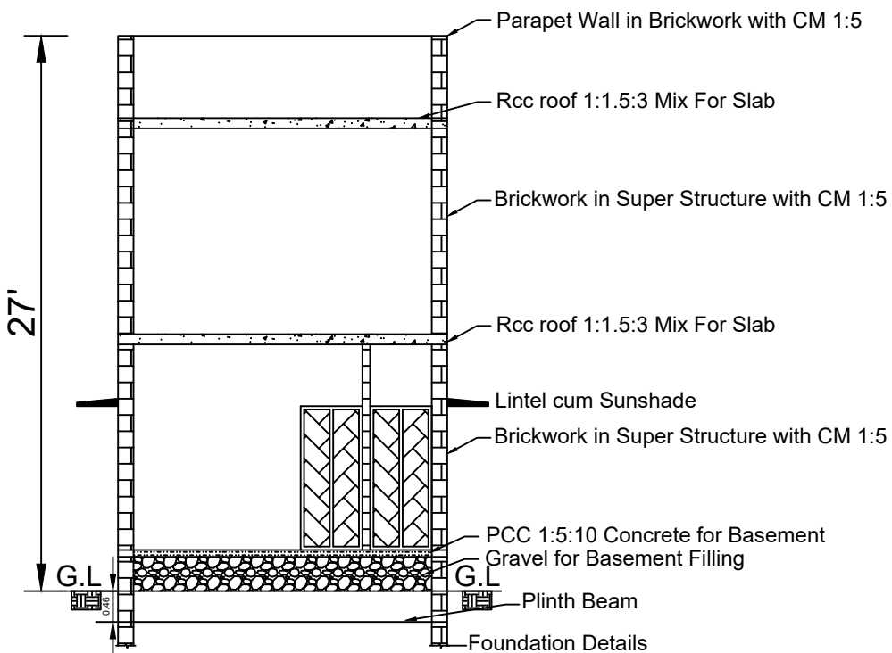
CROSS SECTION ON R-R
