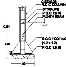
COLUMN DETAILS Size of column = 0.23m x 0.23m Not to scale
