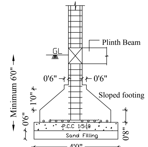
ISOLATED FOOTING / COLUMN DETAIL
