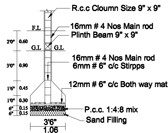
COLUMN DETIAL
