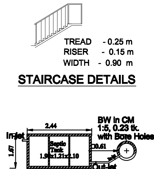
SEPTIC TANK & SOAK PIT
