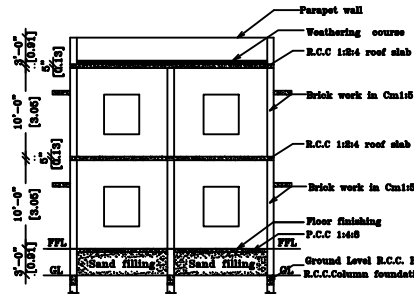
SECTION ON 'SJ'
