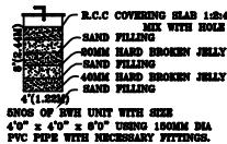
RAIN WATER HARVEST UNIT
