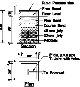
RAINWATER HARVESTING TANK SCALE 1:50
