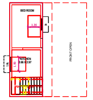
FIRST FLOOR
