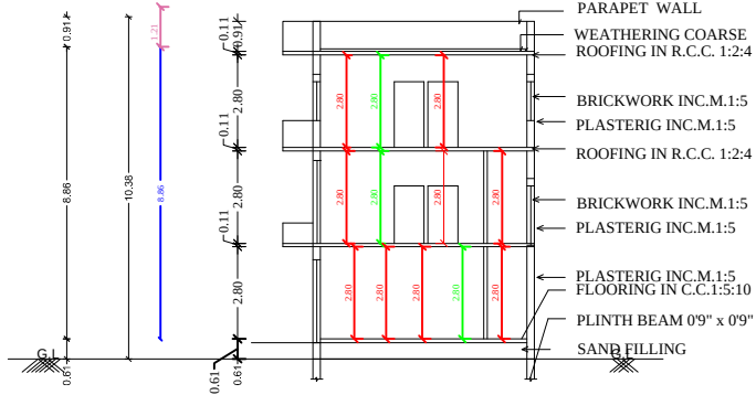
SECTION ON JJ
