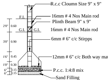
COLUMN DETIAL
