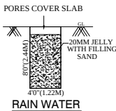
RAIN WATER HARVESTING UNIT NOT TO SCALE
