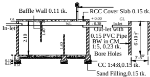
SEPTIC TANK & SOAK PIT
