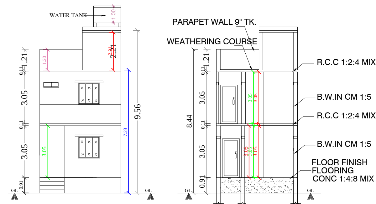
FRONT ELEVATION SECTION : "A-A" (SCALE: 1CM : 1M)
