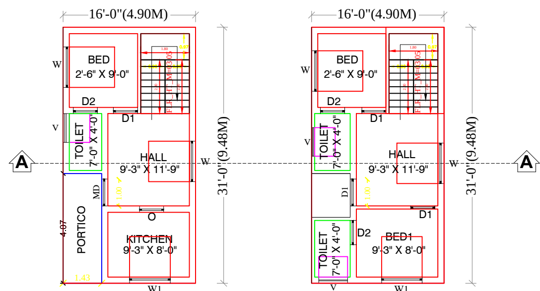
GROUND FLOOR PLAN FIRST FLOOR PLAN AND HEAD ROOM
