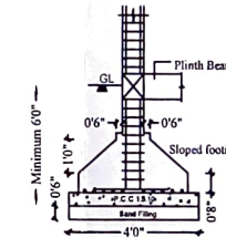
ISOLATED FOOTING / COLUMN DETAIL
