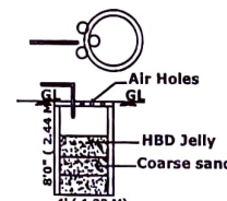
RAIN WATER HARVESTING TANK DETAIL
