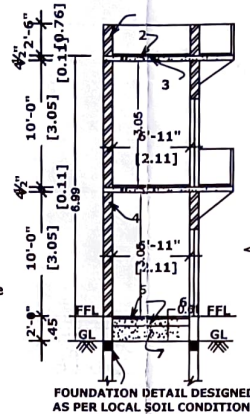
SECTION ON "MD"
