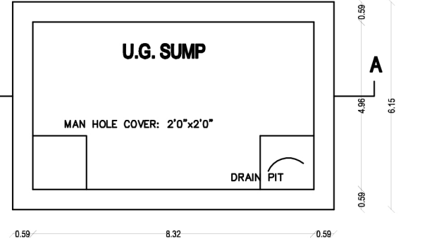
SUMP DETAIL
