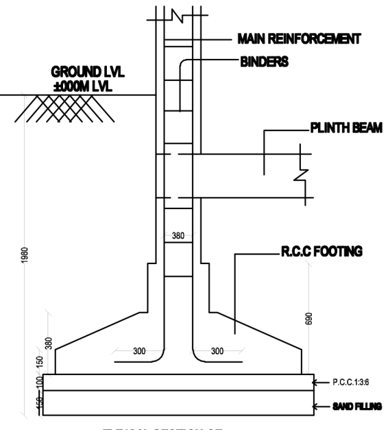
TYPICAL SECTION OF R.C.C COLUMN FOUNDATION SCALE: 1"=2'0"
