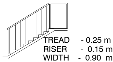
STAIRCASE DETAILS
