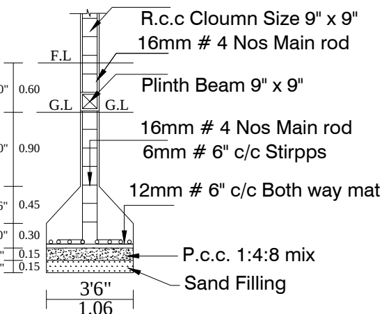
COLUMN DETIAL
