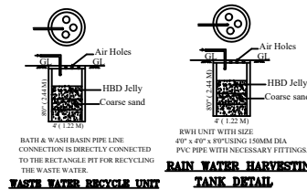
RAIN WATER HARVESTING UNIT
