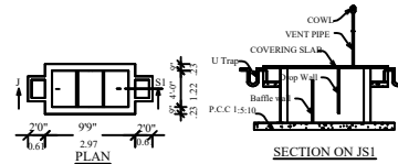
SEPTIC TANK DETAILS
