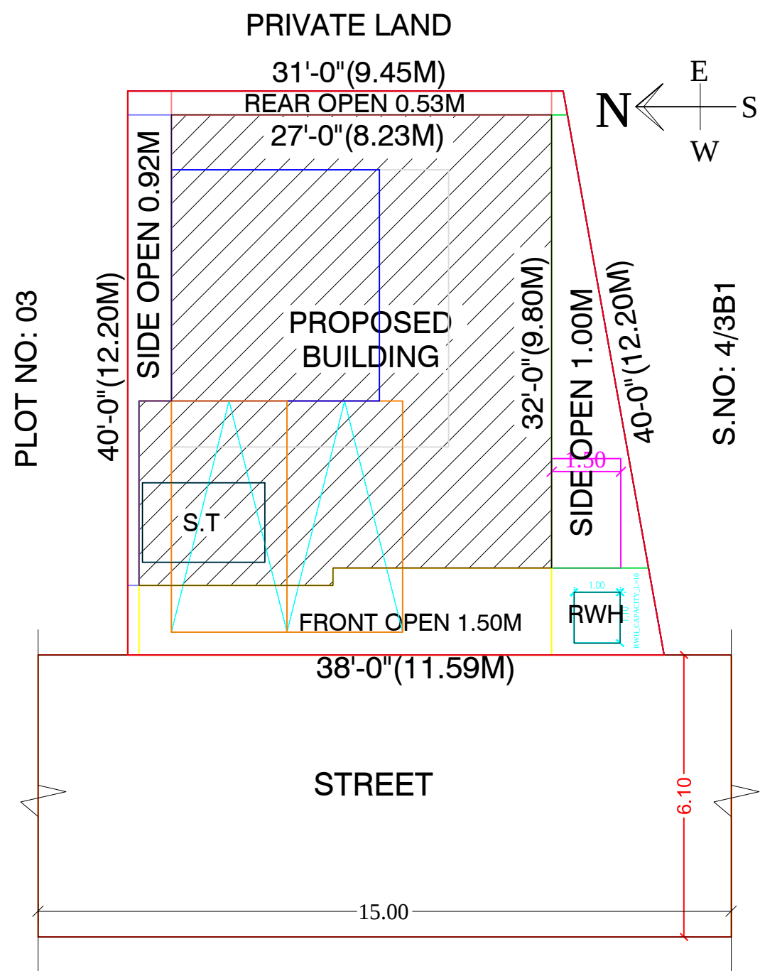
SITE PLAN SCALE: 1CM: 1M
