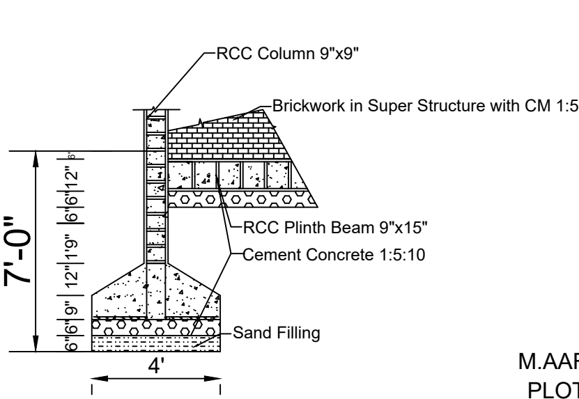
FOUNDATION DETAILS
