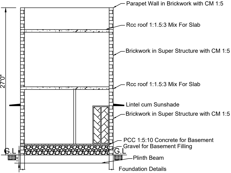
CROSS SECTION ON R-R
