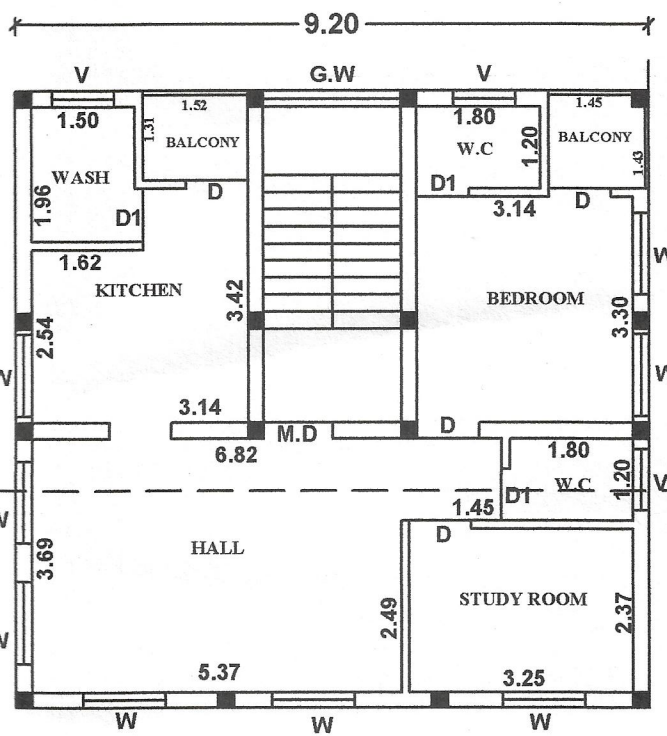
TYPICAL_FLOOR_PLAN=1,2,3
