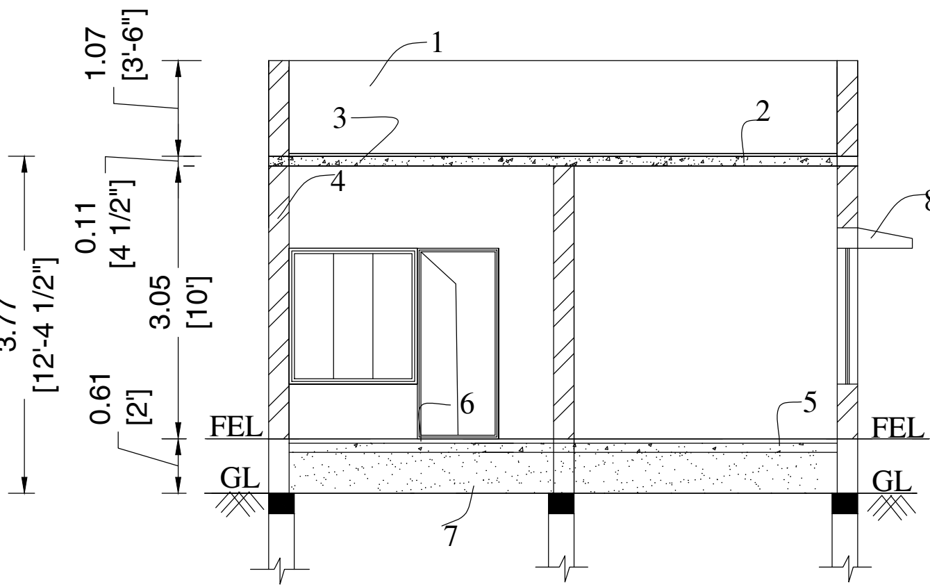
SECTION ON "JS"
