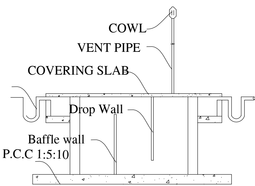
SECTION ON JS1
