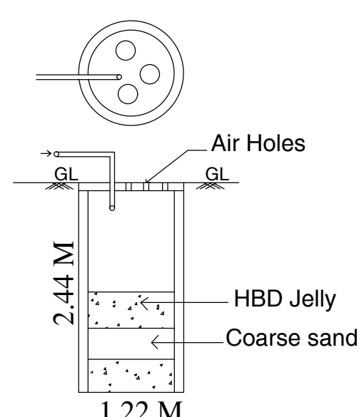
RAIN WATER HARVESTING TANK DETAIL
