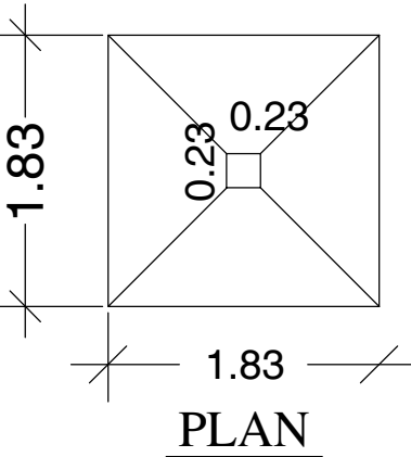
COLUMN DETAILS
