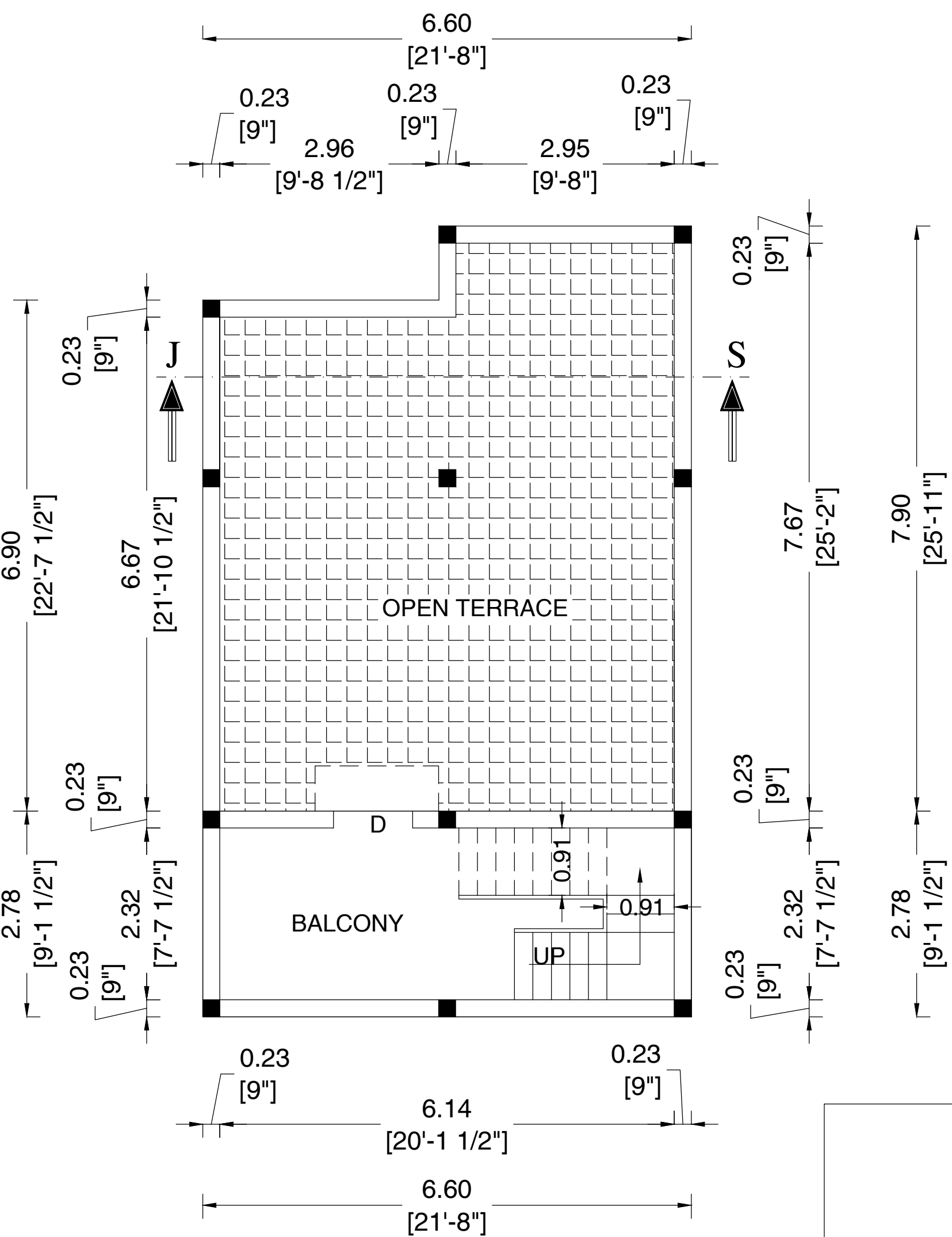
PRO.,HEAD ROOM PLAN
