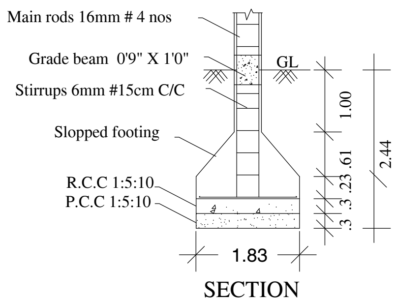
SECTION
