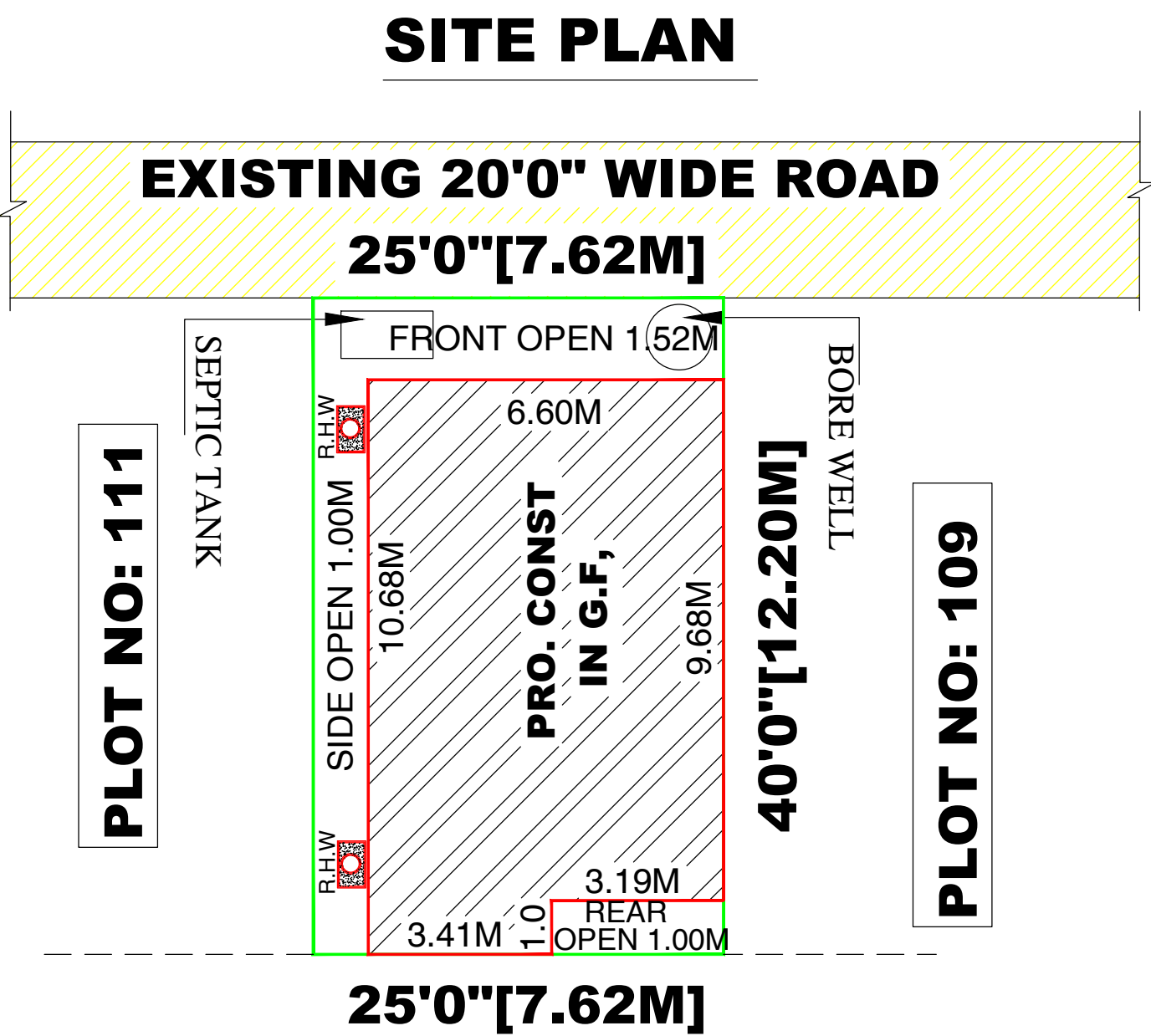
SITE PLAN
