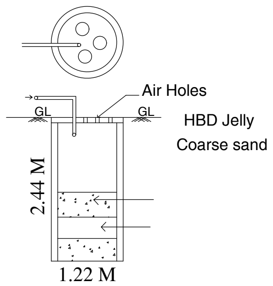
WASTE WATER RECYCLE UNIT
