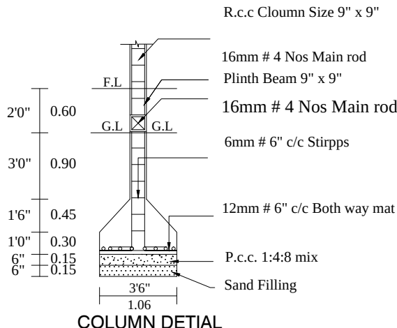
COLUMN DETAIL
