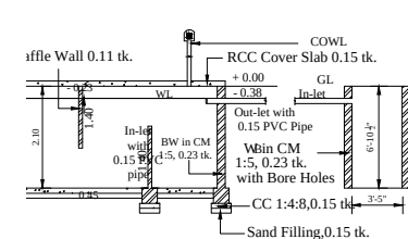
SECTION - SEPTIC TANK & SOAK PIT
