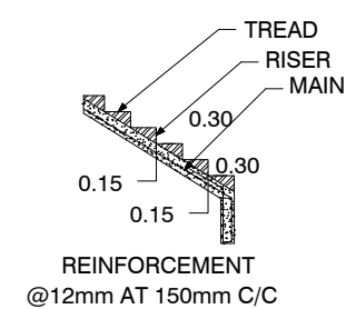
STAIRCASE DETAILS
