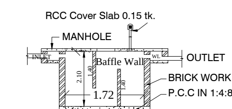
SECTION - SEPTIC TANK
