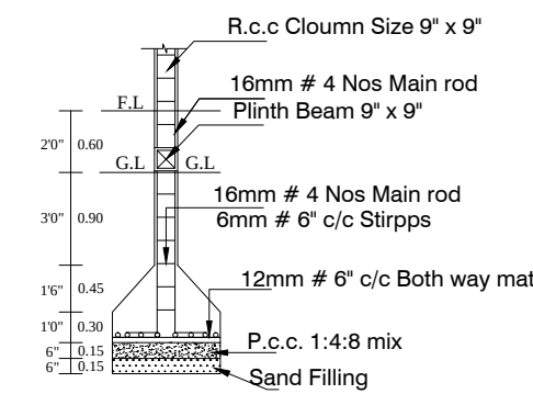
COLUMN DETIAL
