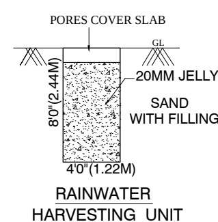
RAINWATER HARVESTING UNIT
