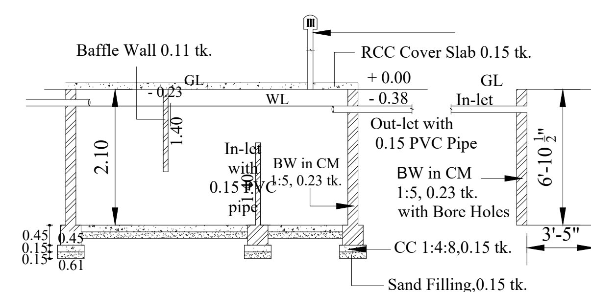
SECTION - SEPTIC TANK &amp; SOAK PIT
