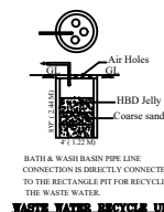
WASTE WATER RECYCLING UNIT
