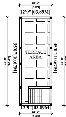
TERRACE FLOOR
