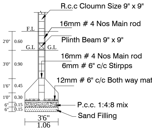
COLUMN DETIAL
