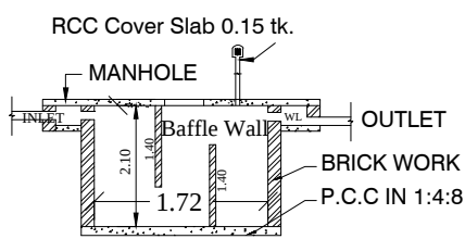
SECTION - SEPTIC TANK
