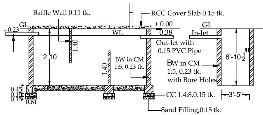
Section - Septic tank & Soak pit
