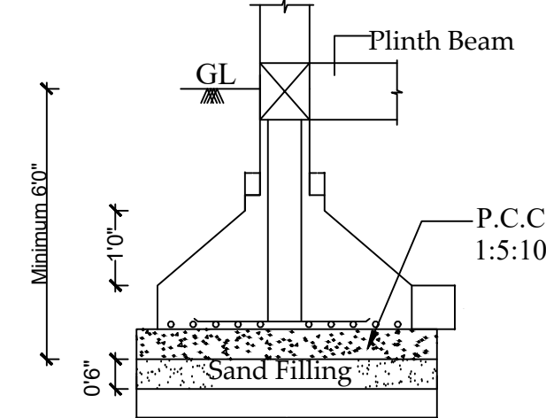
Isolated Footing (5'0"x5'0") (Not to Scale)
