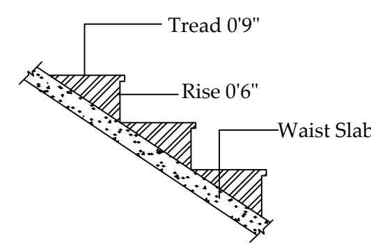
Section of the Staircase Not to Scale
