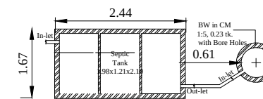
PLAN - SEPTIC TANK & SOAK PIT
