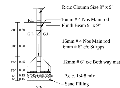
COLUMN DETIAL
