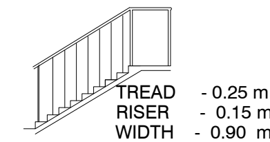
STAIRCASE DETAILS
