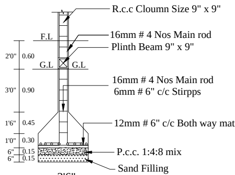
COLUMN DETIAL
