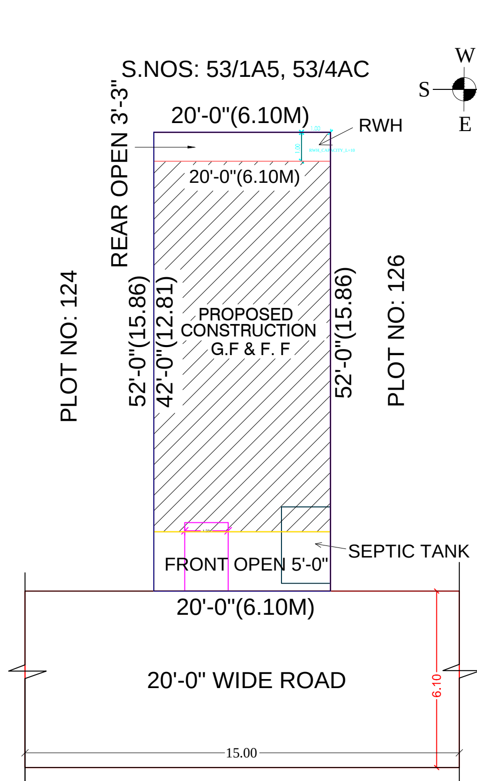
SITE PLAN SCALE: 1CM: 1M
