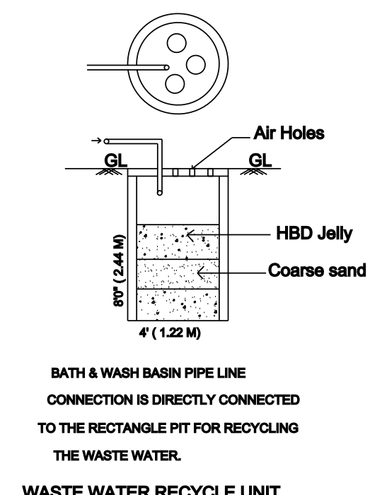
WASTE WATER RECYCLE UNIT
