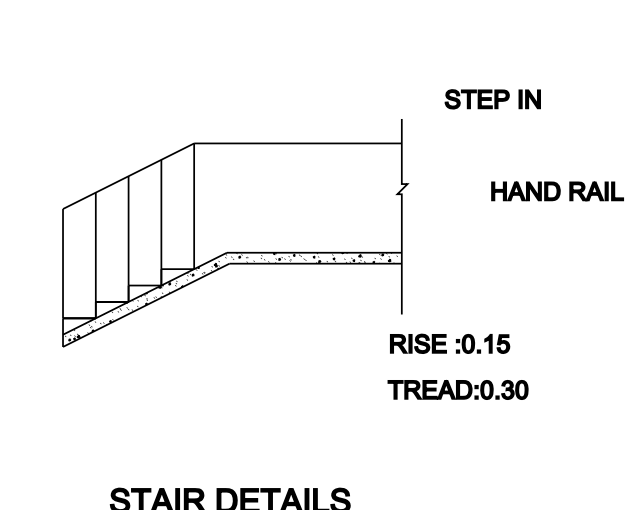
STAIR DETAILS
