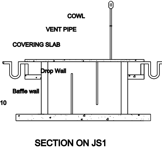
SEPTIC TANK DETAILS Using 'U' type trap 2 Nos in inlet, outlet & vent pipe will be covered with Mosquito proof covering net in inner side and top of vent pipe.
