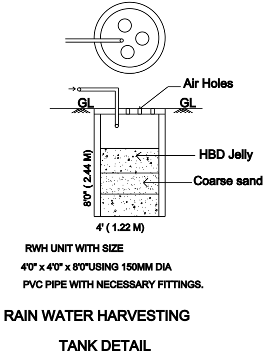
RAIN WATER HARVESTING TANK DETAIL
