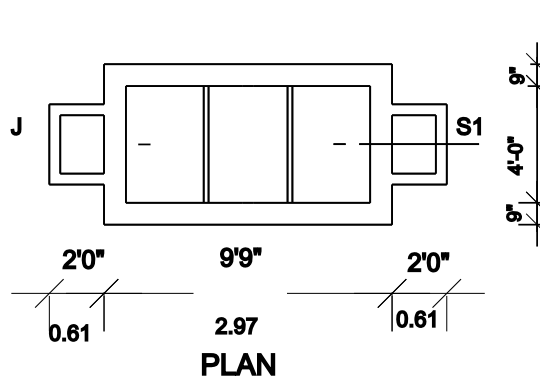
SEPTIC TANK DETAILS Using 'U' type trap 2 Nos in inlet, outlet & vent pipe will be covered with Mosquito proof covering net in inner side and top of vent pipe.
