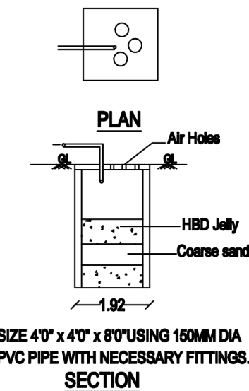
RAIN WATER HARVESTING
