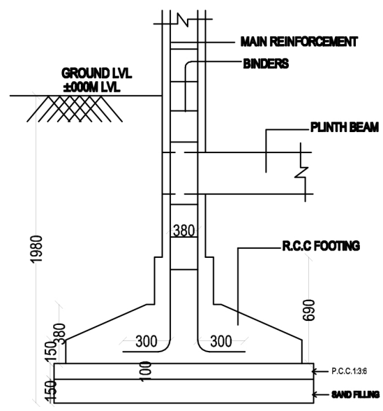
TYPICAL SECTION OF R.C.C COLUMN FOUNDATION SCALE: 1"=2'0"
