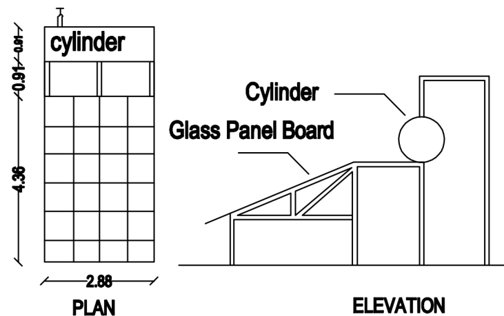
SOLAR ENERGY SYSTEM
