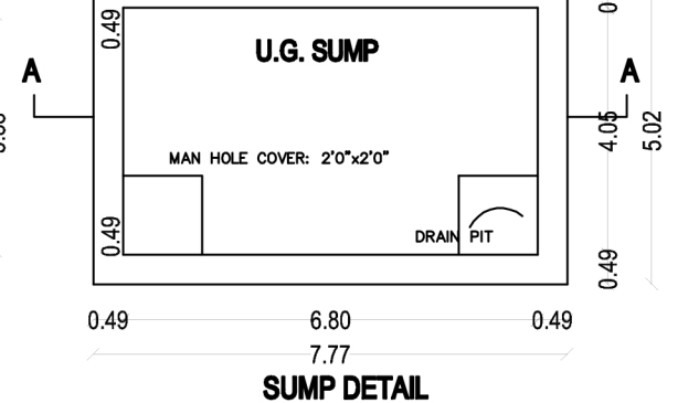
SUMP DETAIL
